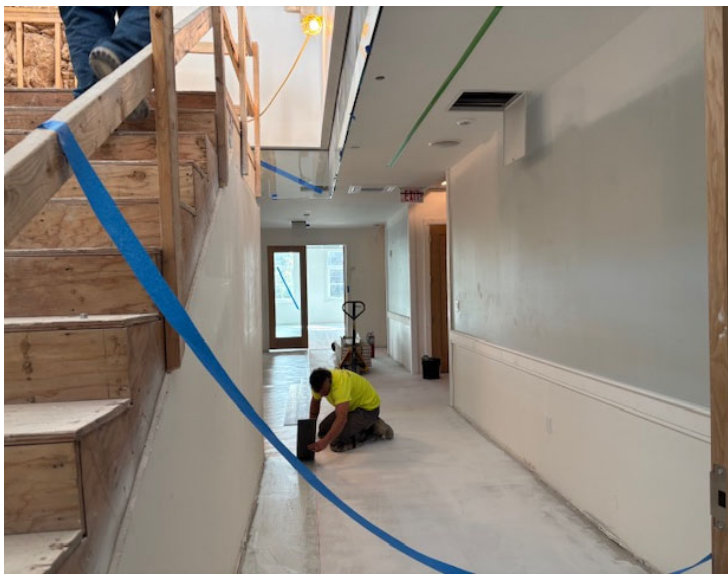
Flooring Ongoing at Main Corridor
