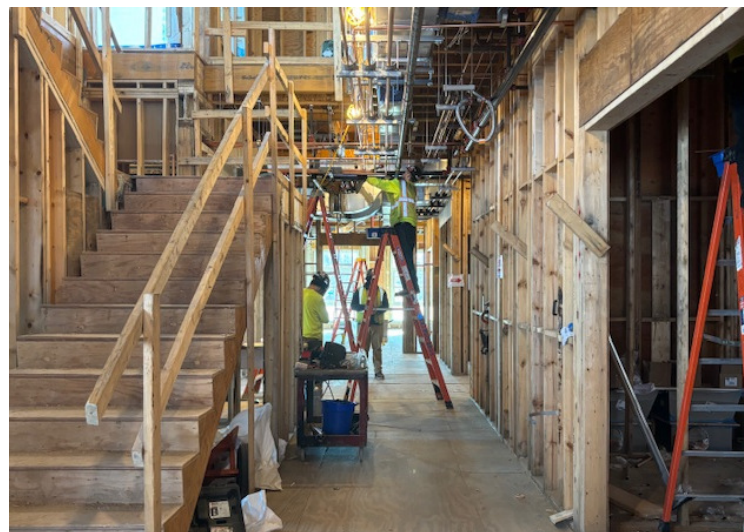
Piping and Conduit Installation in Corridor Ceiling
